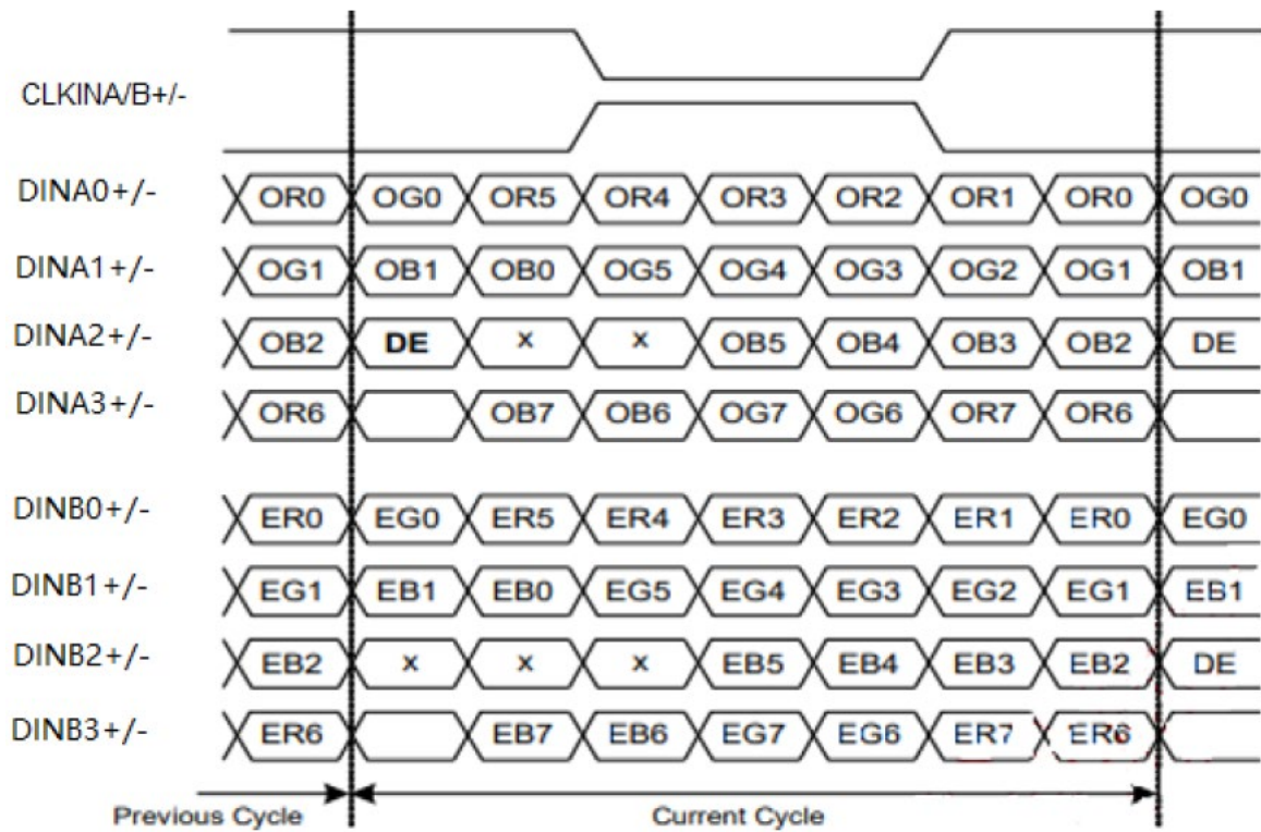
Figure. LVDS data mapping (VESA standard)
