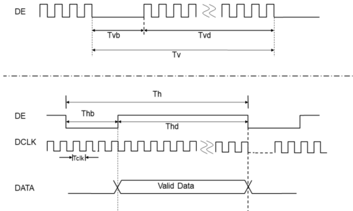
Clock and Data Input Timing Diagram
